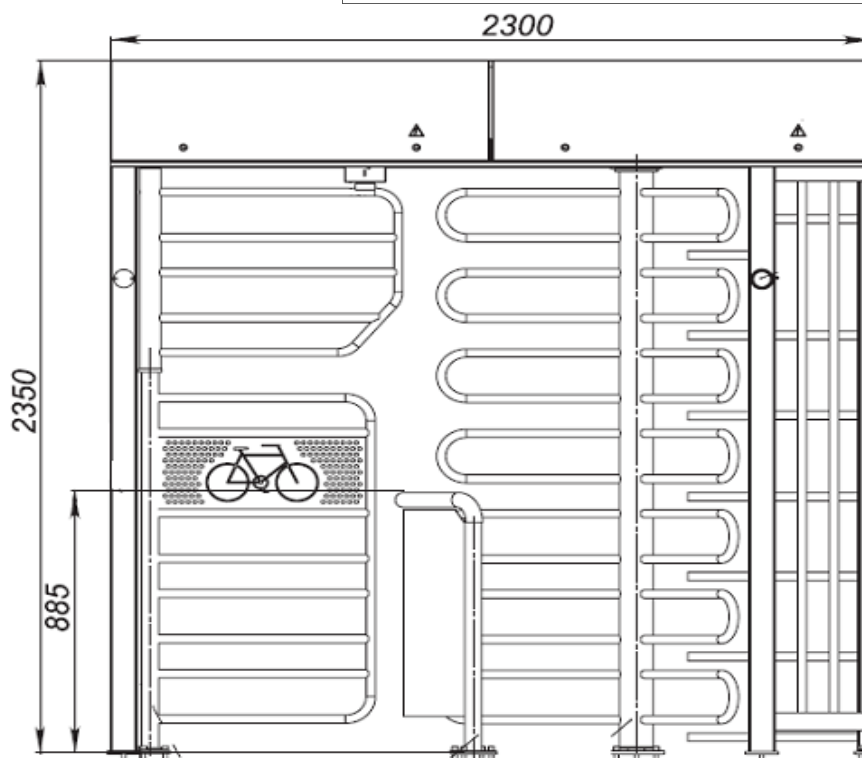
FRONT VIEW
